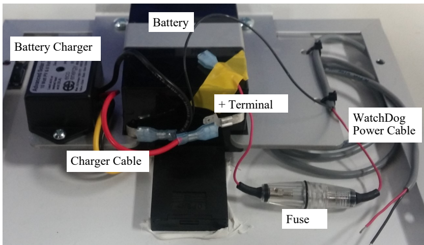
Figure 1: Main Assembly
