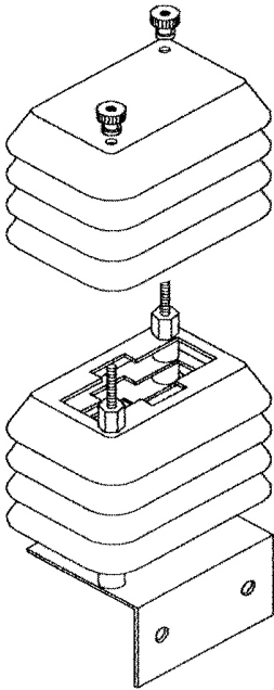
Radiation Shield
